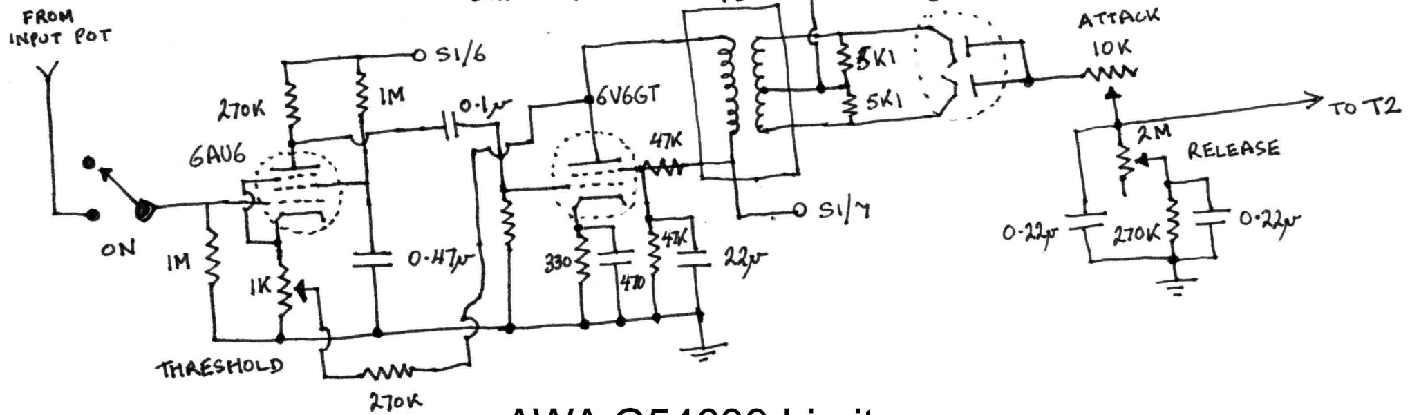
AWA G54639 Limiter MODS BY PROHARMONIC
